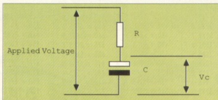
Figure I: R C series circuit
