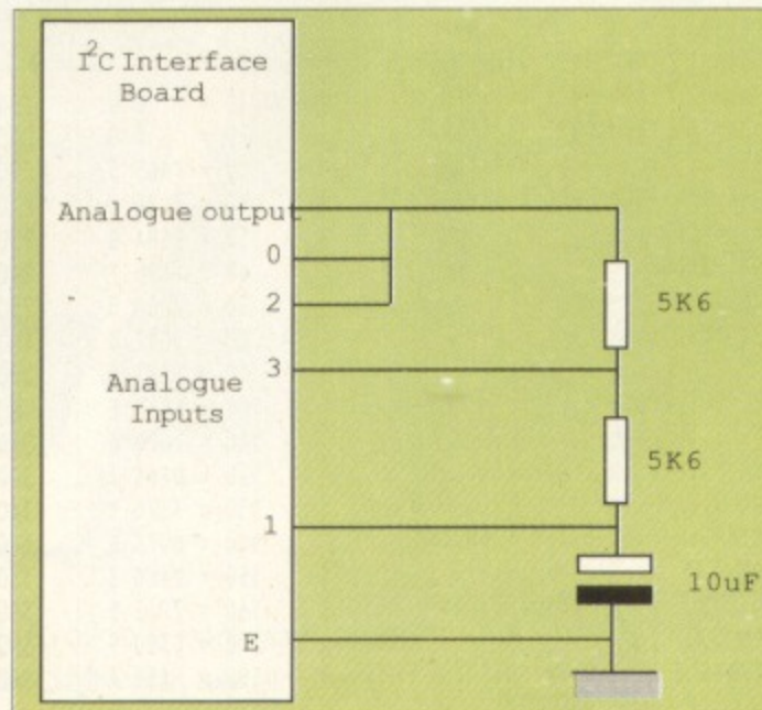
Figure II: The capacitor charging experiment
